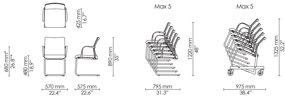
Cantilever - armchair Normal back
