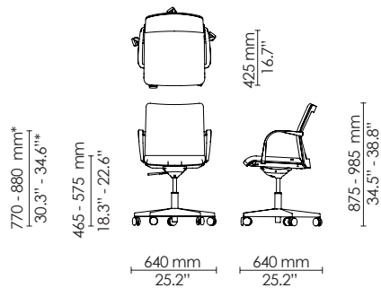
5-star - armchair Normal back
