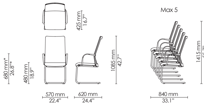
Cantilever - armchair High back
