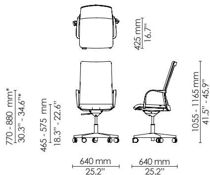
5-star - armchair High back
